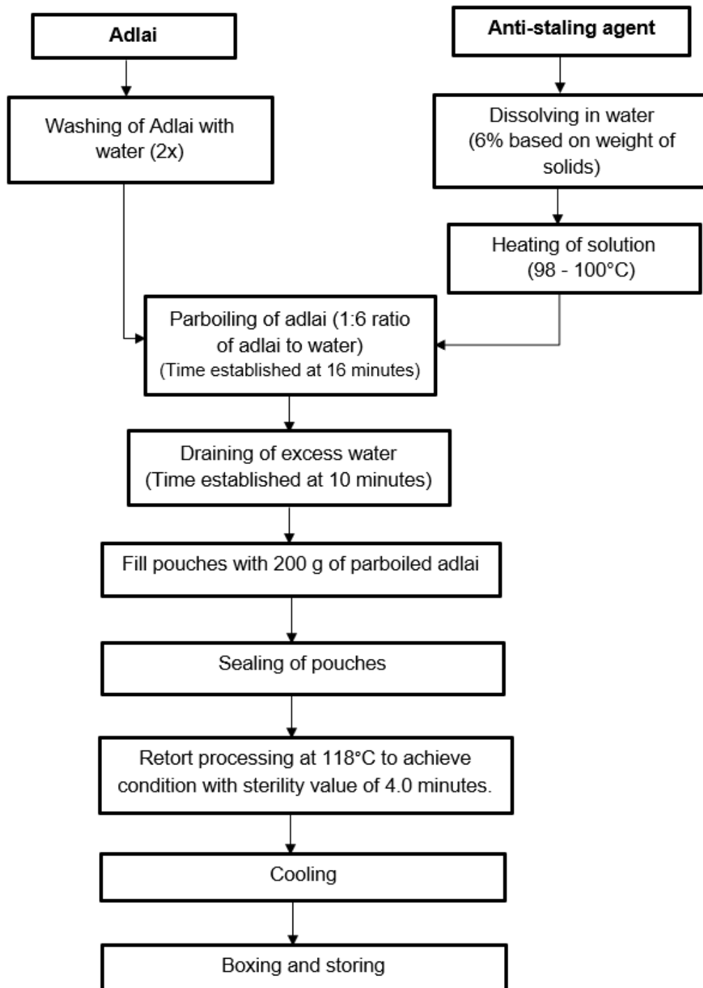
Fig. 1 is a process flow of RTE parboiled adlai
