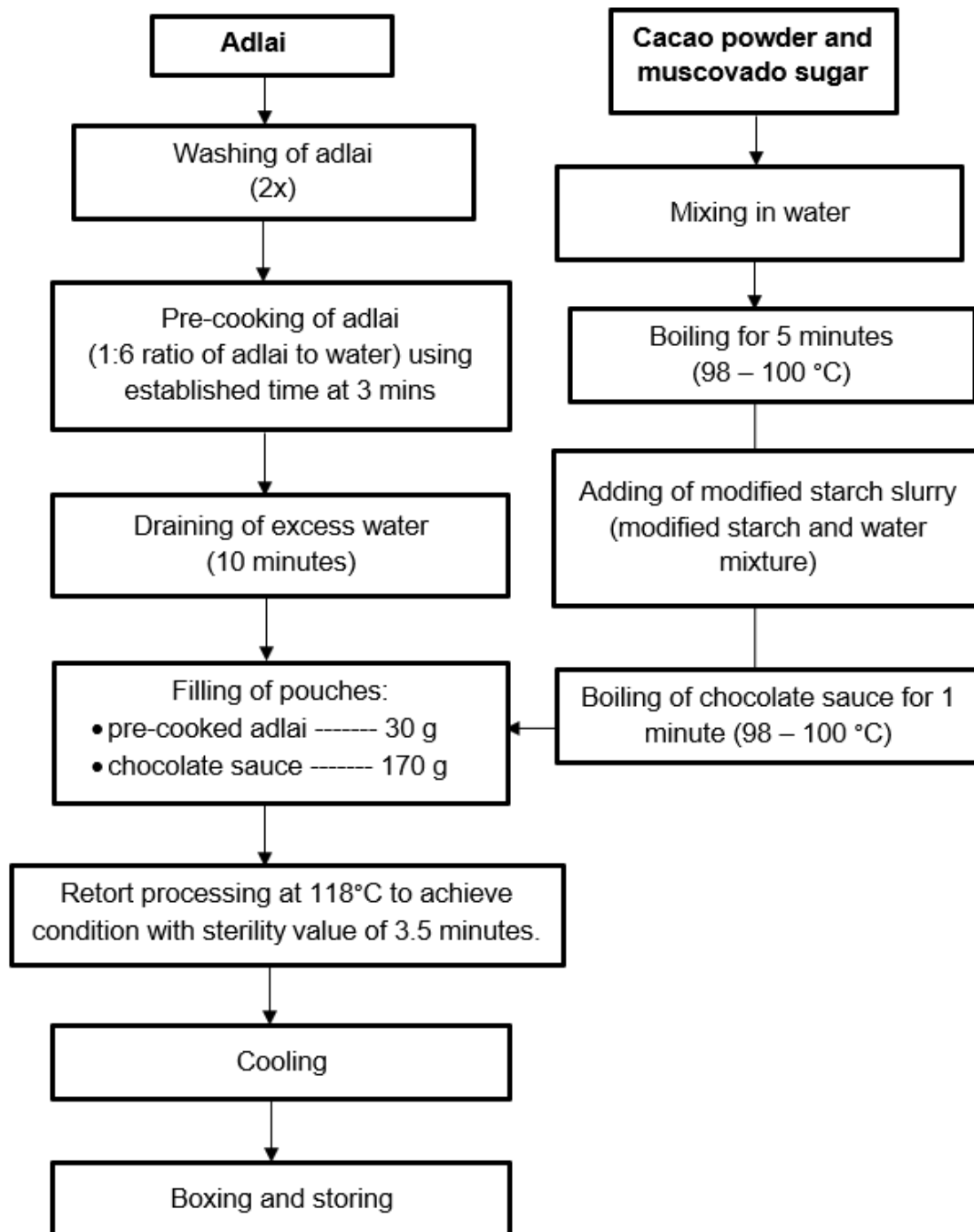
Fig. 1 is a flowchart of a process of producing RTE adlai champorado
